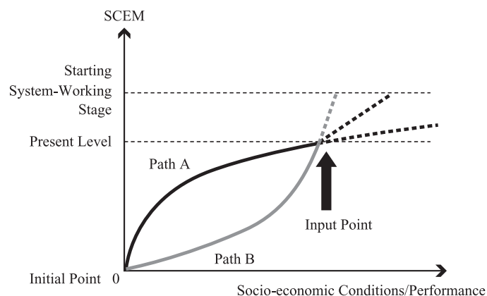
Figure 14 Path analysis
